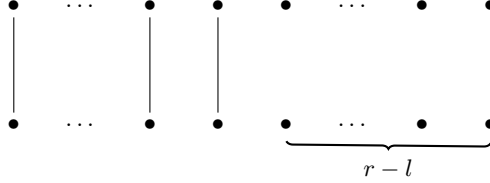
FIGURE 5. The idempotent e_l is defined to be \delta^{r-l} times the diagram above having l propagating blocks.
