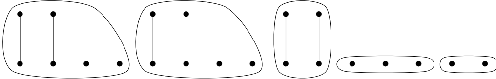
FIGURE 25. The diagram v_{\gamma,\varepsilon} for \gamma = (2^2, 0) and \varepsilon = (3, 2) with a = 2 and b = 3 , obtained via horizontal concatenation as (v_{(2,2)})^{\otimes 2} \otimes v_{(2,0)} \otimes v_{(\emptyset,3)} \otimes v_{(\emptyset,2)} . This diagram is discussed in Example 9.12.
