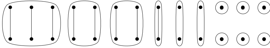
FIGURE 14. The quasi-idempotent e_\vartheta for \vartheta = (3, 2^2, 1, 0^2) in R_{13}(\delta_{\text{in}}, \delta_{\text{out}}) . Note that there are two outer-propagating blocks that are not inner-propagating from the two zero entries. Since 1 \cdot 3 + 2 \cdot 2 + 1 \cdot 1 + 2 \cdot 1 = 10 , there are 3 remaining northern and southern nodes forming singleton outer blocks.
