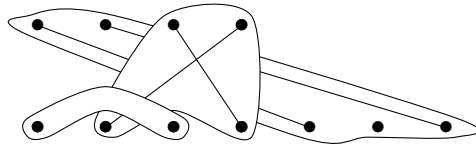
FIGURE 19. Another diagram in V_7^0(2^2) . This ramified diagram can be obtained from that of Figure 18 by acting on the left by ((1, 2), 1_{\mathfrak{S}_2}; (1, 2)) \in \mathfrak{S}_2 \wr \mathfrak{S}_2 . Observe that it cannot be obtained from the ramified diagram of Figure 18 via a right action.
