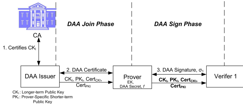
Figure 2: The Rudolph Attack
