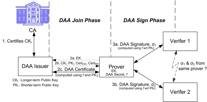
Figure 1: The DAA Scheme
