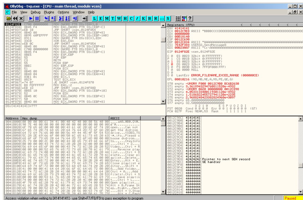
Figure 3.9: Structured exception handler overwrite
