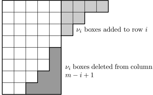
FIGURE 1. Construction of the partition (5^8) \star (4, 2, 1) .
