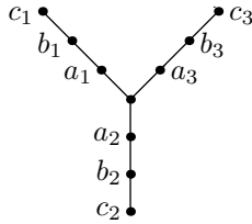
FIGURE 1. The minimal palace T in which the princess can avoid the prince.
