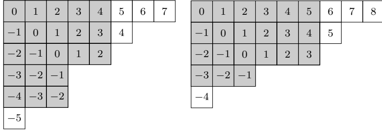
FIGURE 2. The content of the partition obtained from \lambda by deleting a part of size R(\lambda) and inserting it as a new column is C(\lambda) + 1 is obtained by adding 1 to the content of each box of [\lambda] ; this can be seen here by comparing the shaded and unshaded boxes.
